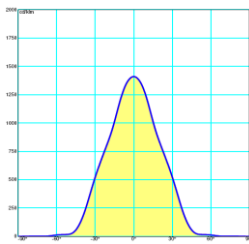
SYMMETRIC OPTIC - MB 2x30°
